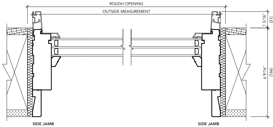
METAL CLAD TRIPLE 6 9/16" (166 mm)
