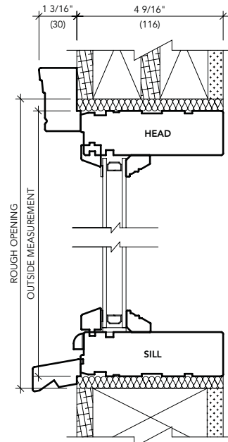
WOOD DOUBLE 4 9/16" (116 mm)
