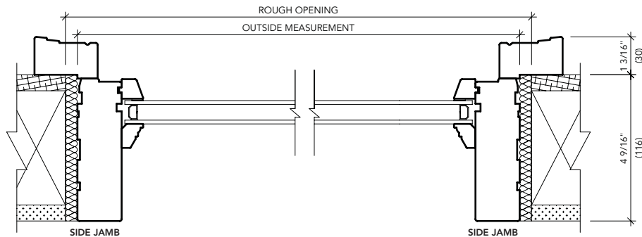
WOOD DOUBLE 4 9/16" (116 mm)
