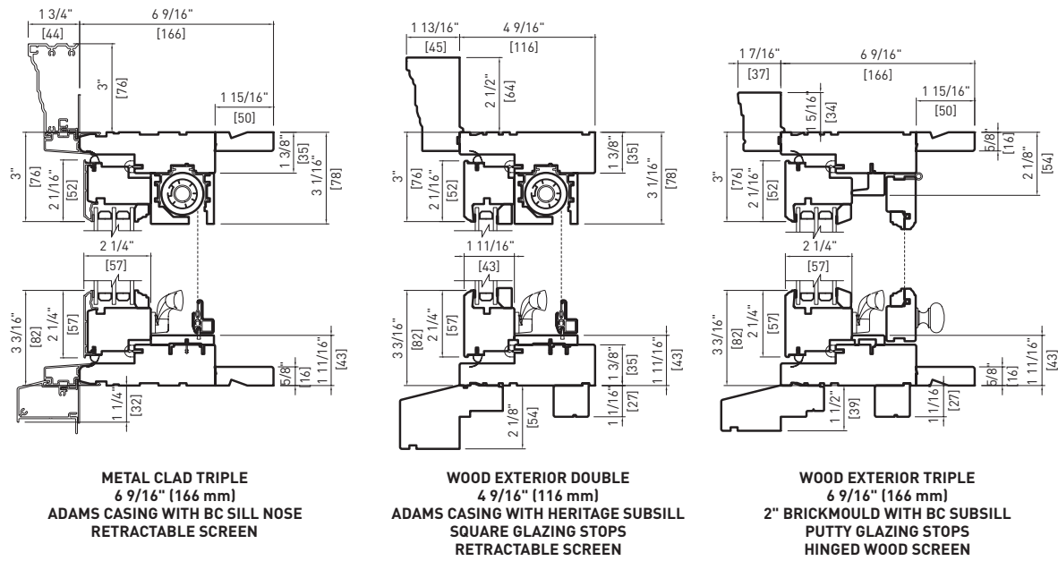
Head & Sill Detail
