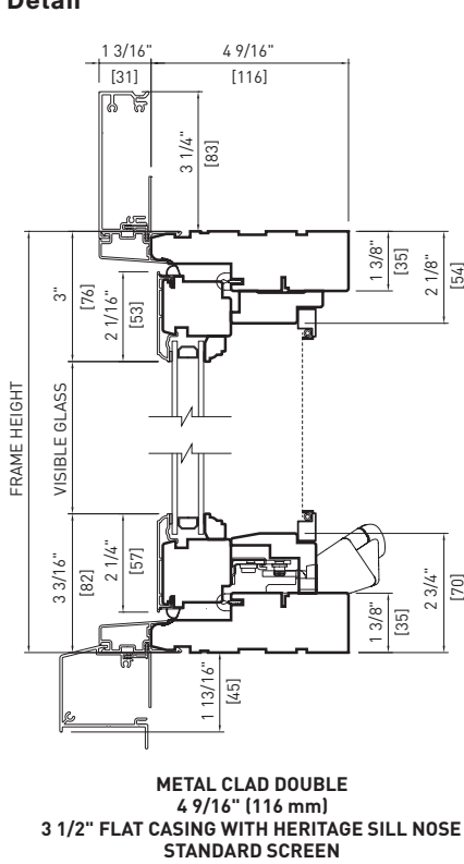
Head & Sill Detail
