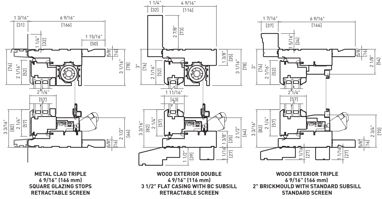
Head & Sill Detail
