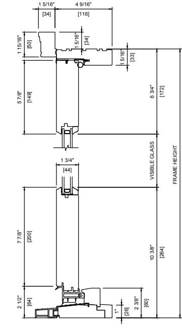
WOOD EXTERIOR DOUBLE 4 9/16" (116mm) 2" BRICKMOULD
