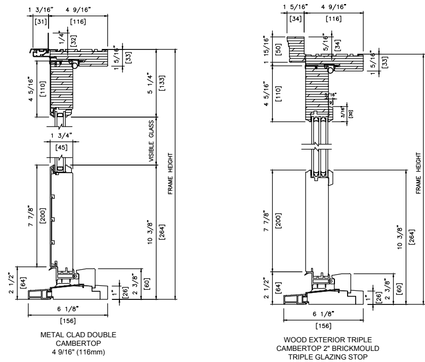
Head & Sill Detail
