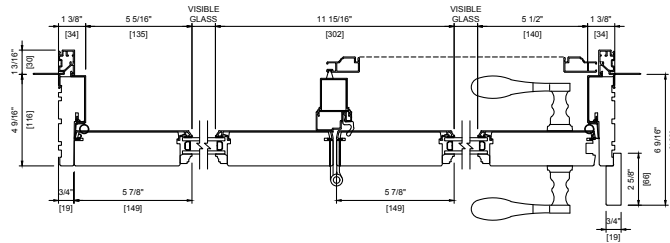
METAL CLAD DOUBLE TWO PANEL
