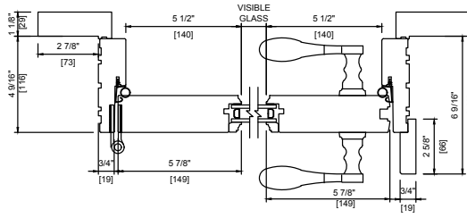
NON CLAD DOUBLE ONE PANEL 3 1/2" FLAT CASING
