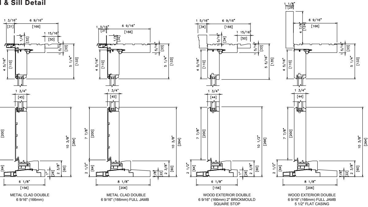
Head & Sill Detail
