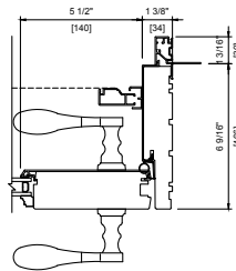
METAL CLAD DOUBLE 6 9/16" (166 mm) FULL JAMB
