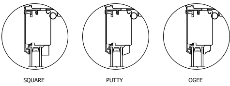
Glazing Stop Profiles
