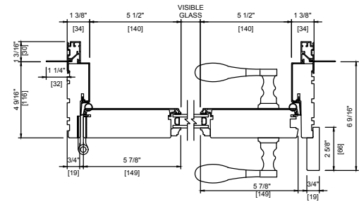
METAL CLAD DOUBLE ONE PANEL
