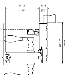
WOOD EXTERIOR DOUBLE 6 9/16" (166 mm) 2" BRICKMOULD
