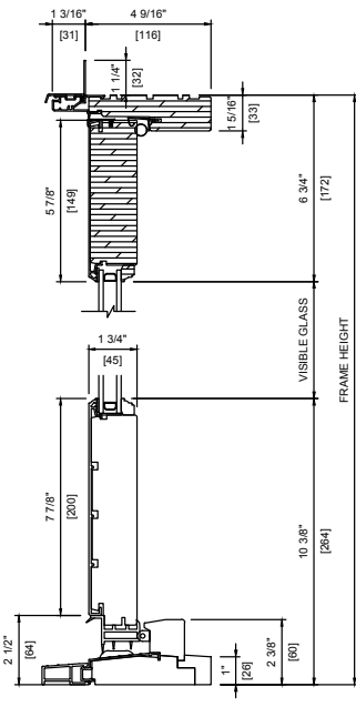
CAMBERTOP METAL CLAD DOUBLE 4 9/16" (116mm)
