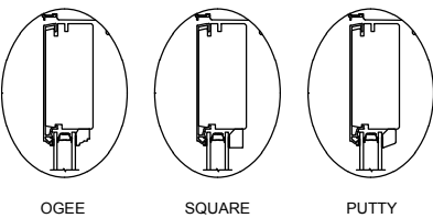
Glazing Stop Profiles
