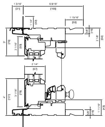
METAL CLAD TRIPLE 6 9/16" (166mm) HINGED WOOD SCREEN
