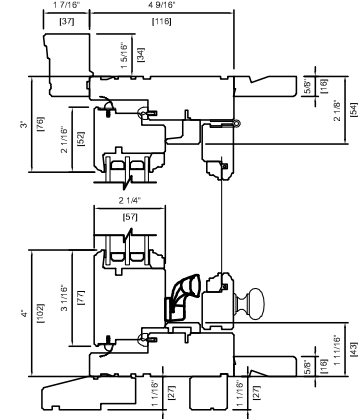
NON CLAD TRIPLE 6 9/16" (166mm) HINGED WOOD SCREEN 2" BRICKMOULD STANDARD SUBSILL
