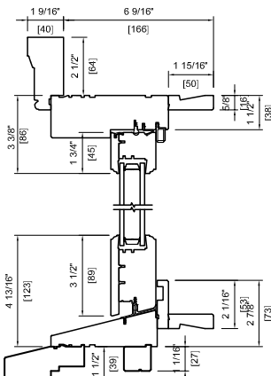
WOOD EXTERIOR DOUBLE 6 9/16" (166 mm) WILLIAMSBURG BC SUB SILL
