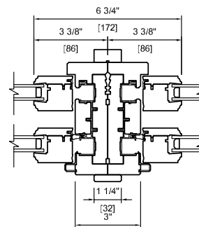
WOOD EXTERIOR
