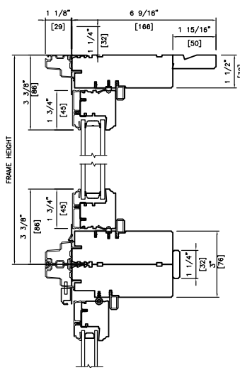
METAL CLAD GRAND SASH DOUBLE 6 9/16" (166 mm)
