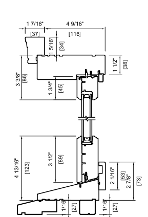
WOOD EXTERIOR DOUBLE 4 9/16" (116 mm) 2" BRICKMOULD STANDARD SUB SILL
