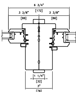
WOOD EXTERIOR
