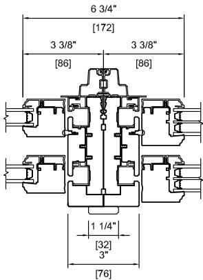
Mull Detail
