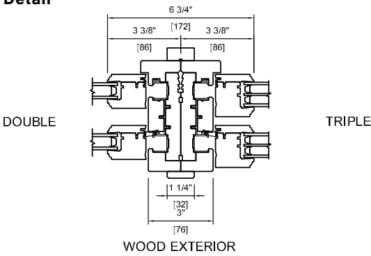
Mull Detail
