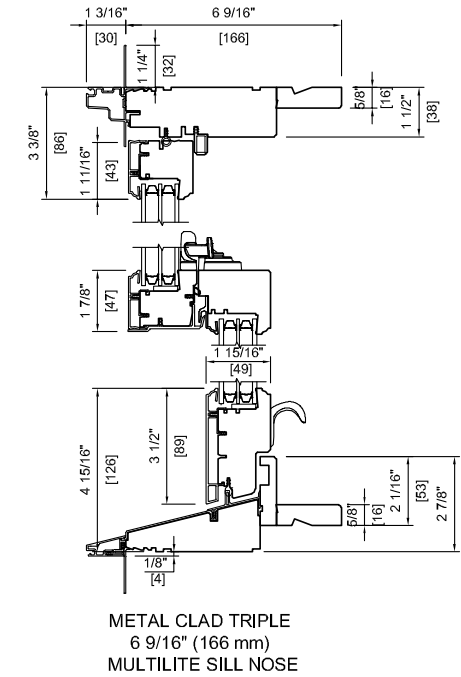
Head & Sill Detail
