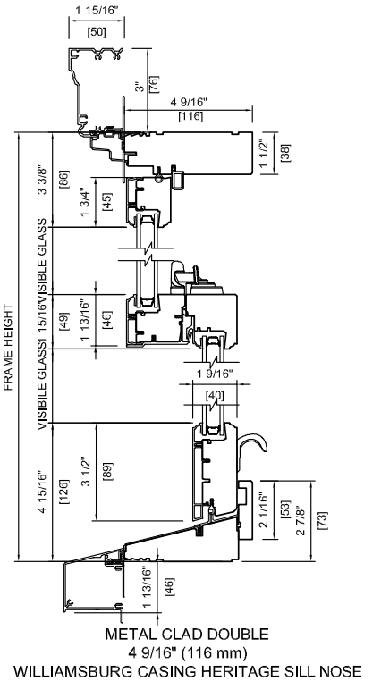
Head & Sill Detail
