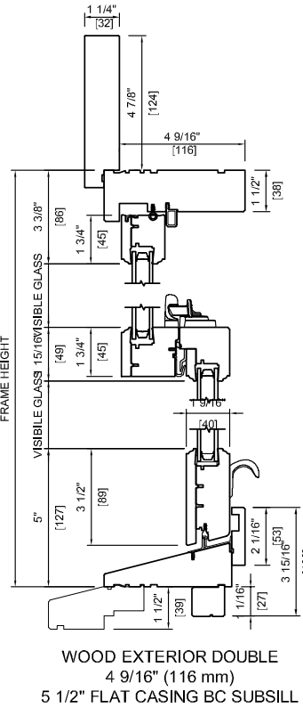
Head & Sill Detail
