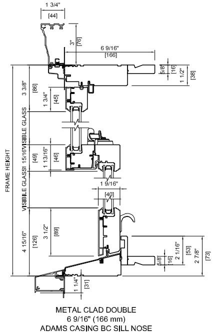
Head & Sill Detail
