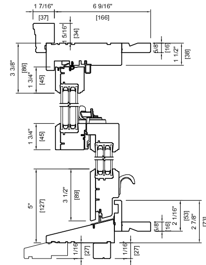
WOOD EXTERIOR TRIPLE 6 9/16" (166 mm) 2" BRICKMOULD STANDARD SUBSILL
