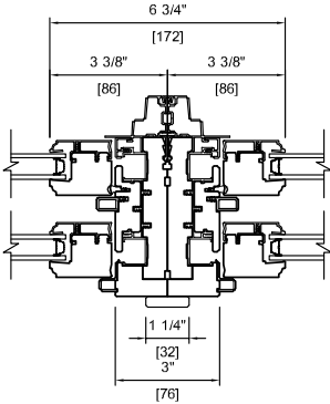
Mull Detail
