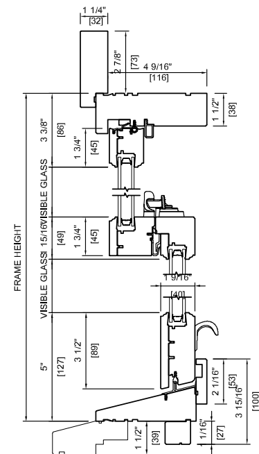
WOOD EXTERIOR DOUBLE 4 9/16" (116 mm) 3 1/2" FLAT CASING BC SUBSILL
