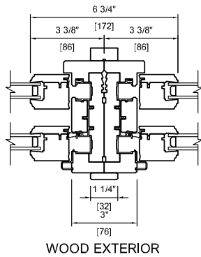
Mull Detail
