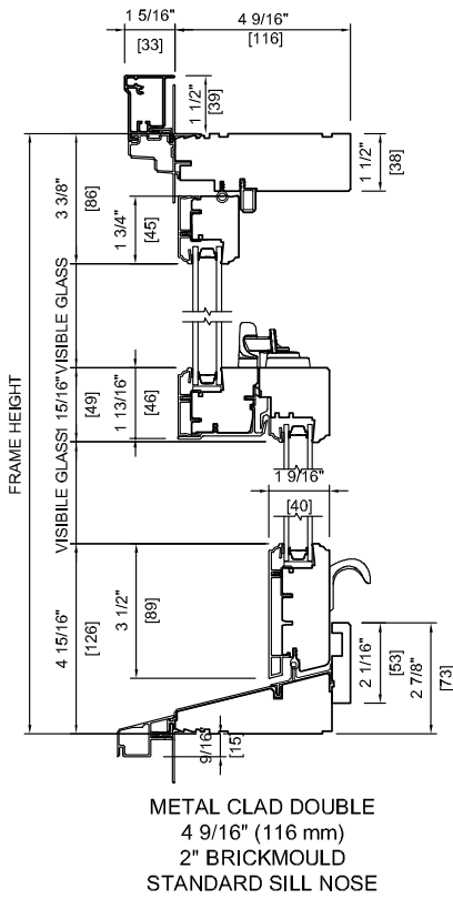
Head & Sill Detail
