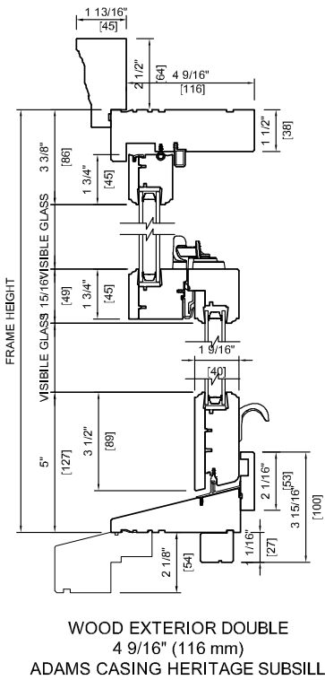
Head & Sill Detail
