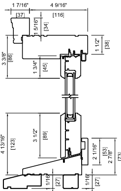
WOOD EXTERIOR DOUBLE 4 9/16" (116 mm) 2" BRICKMOULD STANDARD SUB SILL
