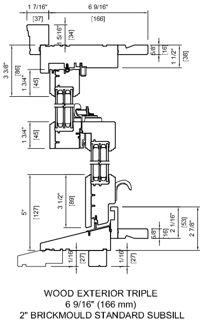
Head & Sill Detail
