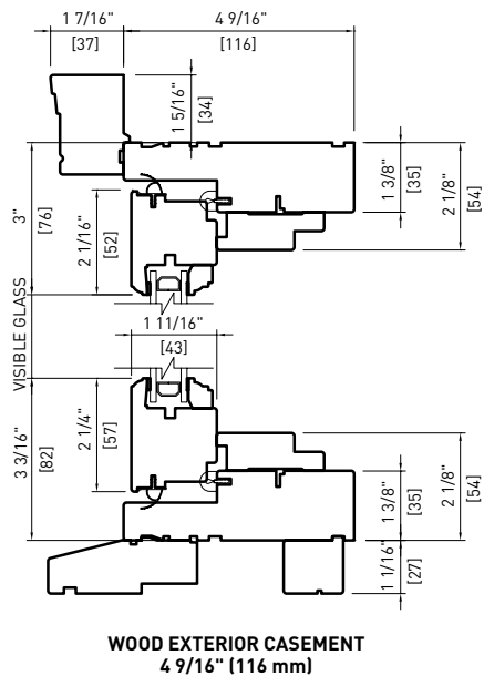
Head & Sill Detail
