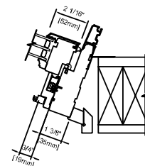
STRAIGHT WALL METAL CLAD CASEMENT 4 9/16" (116 mm) JAMB
