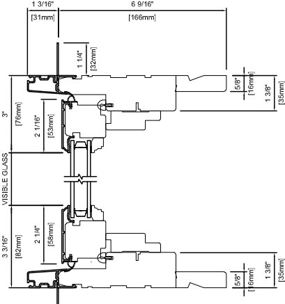
METAL CLAD CASEMENT 6 9/16" (166mm)
