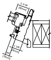
STRAIGHT WALL METAL CLAD CASEMENT 4 9/16" (116 mm) JAMB
