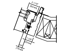
FRAMED WALL METAL CLAD CASEMENT 4 9/16" (116 mm) JAMB
