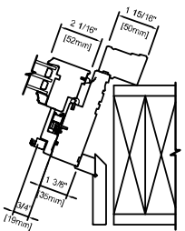
STRAIGHT WALL WOOD CASEMENT 6 9/16" (166 mm) JAMB
