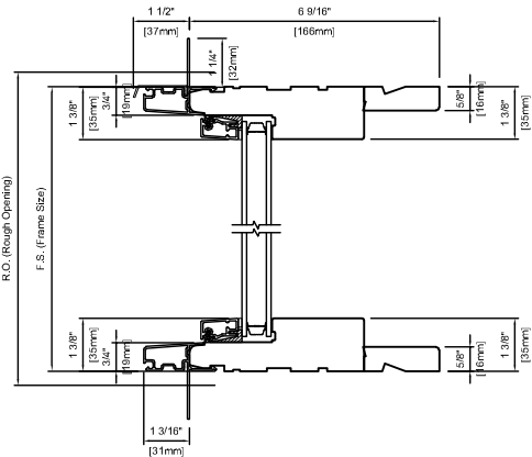
METAL CLAD PICTURE 6 9/16" (166mm)
