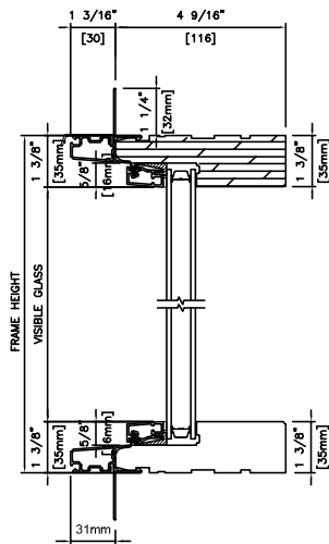
METAL CLAD PICTURE (DUAL GLAZED) 4 9/16" (116mm)
