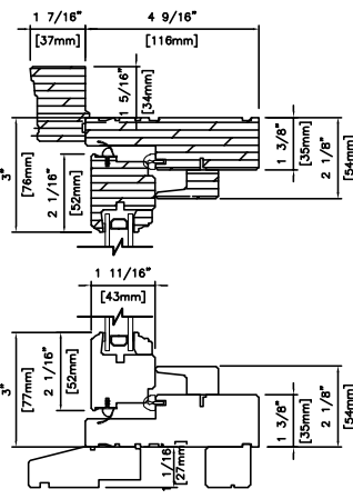
WOOD CASEMENT (DUAL GLAZED) 4 9/16" (116mm) PUSH OUT MOULDINGS 2" BRICKMOULD WITH STANDARD SUBSILL
