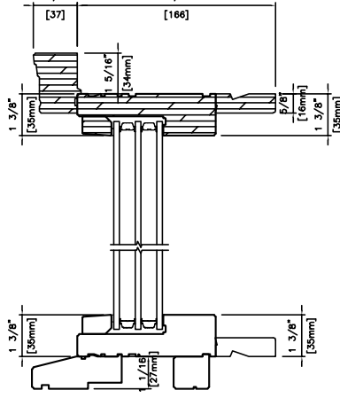
WOOD PICTURE (TRIPLE GLAZED) 6 9/16" (166mm) 2" BRICKMOULD WITH STANDARD SUBSILL
