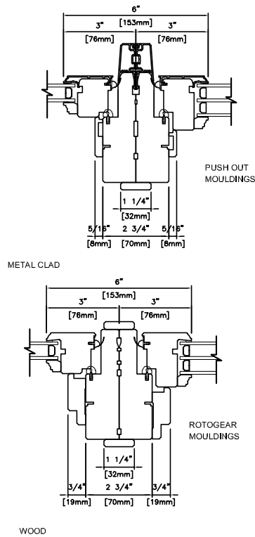
WOOD
