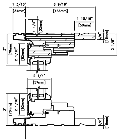
METAL CLAD CASEMENT (TRIPLE GLAZED) 6 9/16" (166mm) ROTOGEAR MOULDINGS
