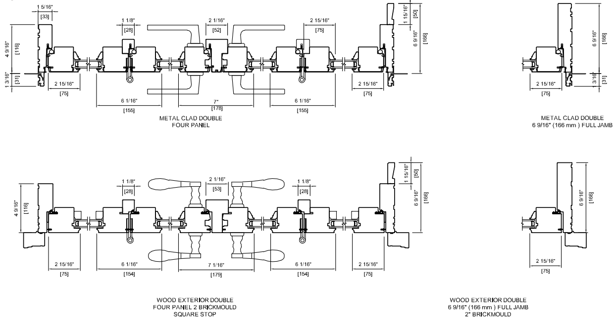
Plan View
