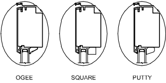
Glazing Stop Profiles
