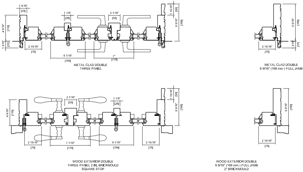
Glazing Stop Profiles
