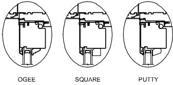
Glazing Stop Profiles
