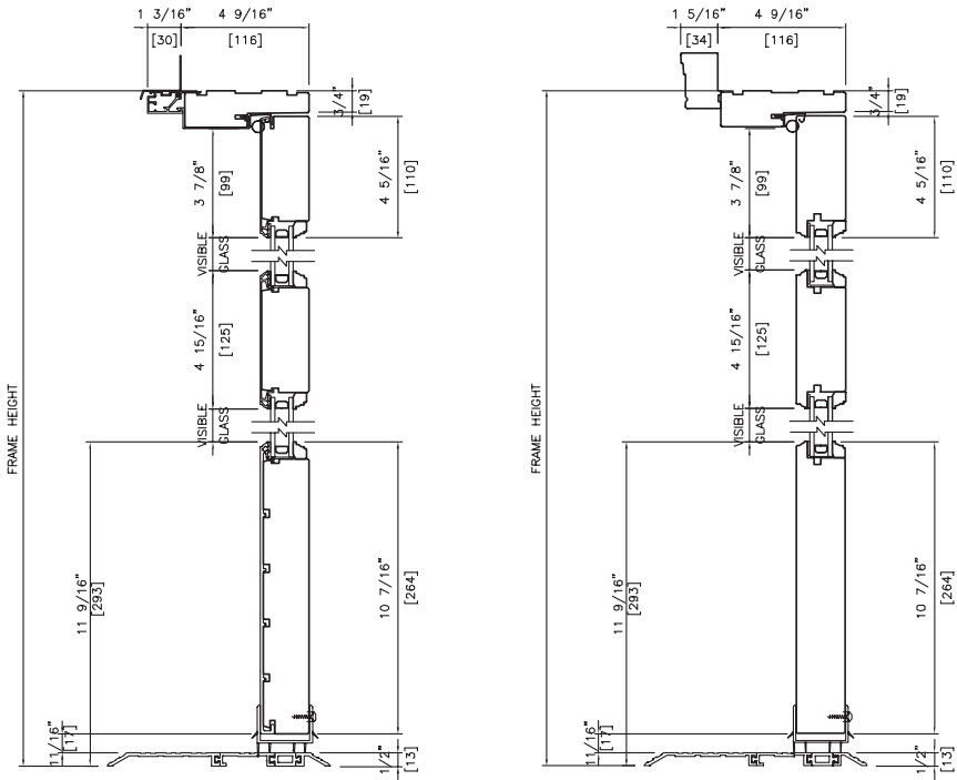
Head & Sill Detail
