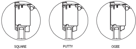
Glazing Stop Profiles
