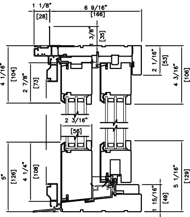
METAL CLAD TRIPLE 6 9/16" (166mm)
