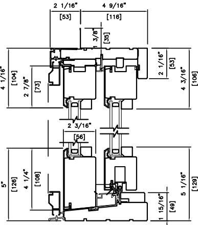
METAL CLAD DOUBLE 4 9/16" (116mm)
