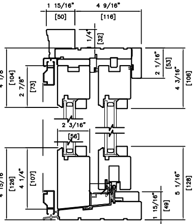
WOOD EXTERIOR DOUBLE 4 9/16" (116mm) 2" BRICKMOULD
