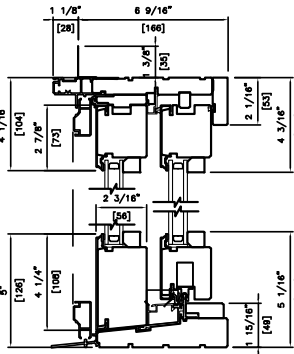
METAL CLAD DOUBLE 6 9/16" (166mm)
