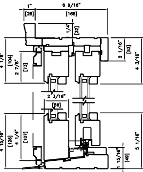
WOOD EXTERIOR DOUBLE 6 9/16" (166mm) 2" BRICKMOULD
