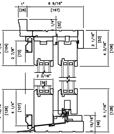
WOOD EXTERIOR TRIPLE 6 9/16" (166mm) 2" BRICKMOULD
