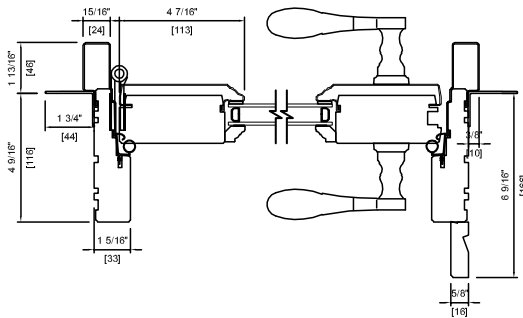
CYPRIUM DOUBLE ONE PANEL 4 9/16" (116mm) / 6 9/16" (166mm)
