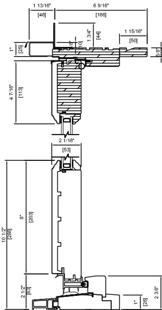
CYPRIUM DOUBLE 6 9/16" (166mm)
