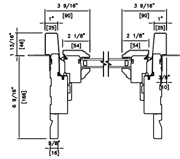
CYPRIUM DOUBLE 6 9/16" (166mm) MATCH PUSHOUT JAMB MOULDING
