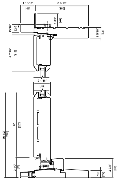
CYPRIUM DOUBLE 6 9/16" (166mm) FULL JAMB
