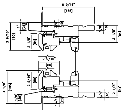
CYPRUM DOUBLE 6 9/16" (166mm) HINGED WOOD SCREEN
