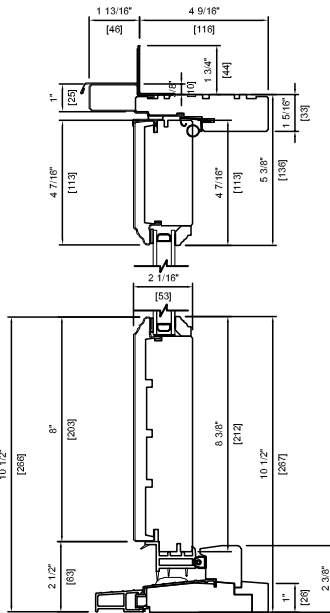
CYPRIUM DOUBLE 4 9/16" (116mm)
