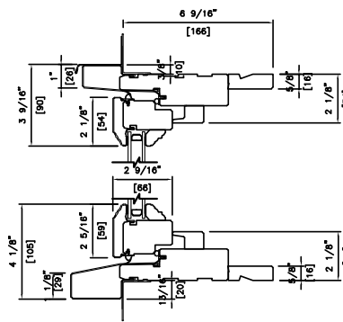
CYPRIUM DOUBLE 6 9/16" (166mm) MATCH PUSHOUT JAMB MOULDING
