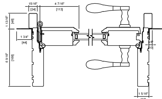
CYPRIUM DOUBLE ONE PANEL 6 9/16" (166mm)
