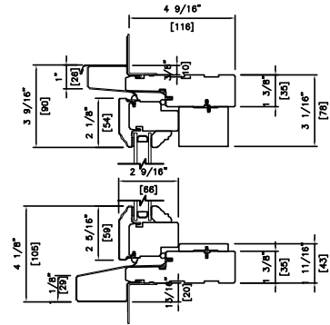
CYPRIUM DOUBLE 4 9/16" (116mm) MATCH RETRACTABLE SCREEN JAMB MOULDING
