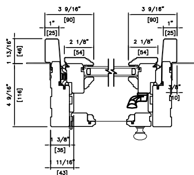
CYPRUM DOUBLE 4 9/16" (116mm) HINGED WOOD SCREEN
