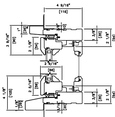
CYPRUM DOUBLE 4 9/16" (116mm) HINGED WOOD SCREEN
