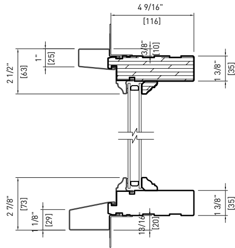
CYPRIMUM DOUBLE 4 9/16" [116 mm]
