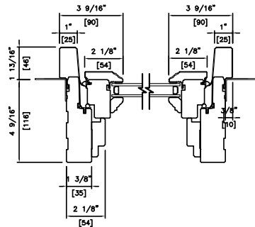
CYPRIUM DOUBLE 4 9/16" (116mm) MATCH STANDARD JAMB MOULDING
