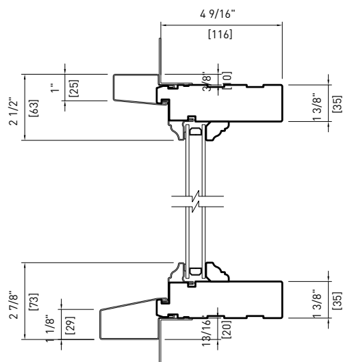
CYPRIUM DOUBLE 4 9/16" (116 mm)
