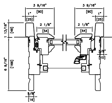
CYPRUM DOUBLE 6 9/16" (166mm) RETRACTABLE SCREEN
