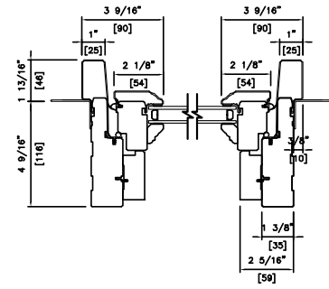
CYPRIUM DOUBLE 4 9/16" (116mm) MATCH RETRACTABLE SCREEN JAMB MOULDING
