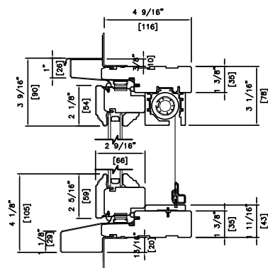
CYPRUM DOUBLE 4 9/16" (116mm) RETRACTABLE SCREEN
