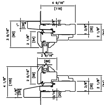
CYPRIUM DOUBLE 4 9/16" (116mm) MATCH STANDARD JAMB MOULDING
