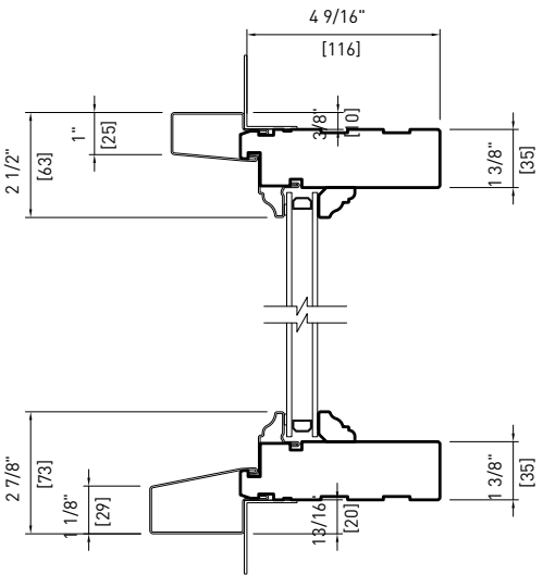
CYPRIMUM DOUBLE 4 9/16" (116 mm)
