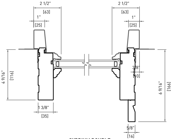
CYPRIMUM DOUBLE 4 9/16" (116 mm) / 6 9/16" (166 mm)
