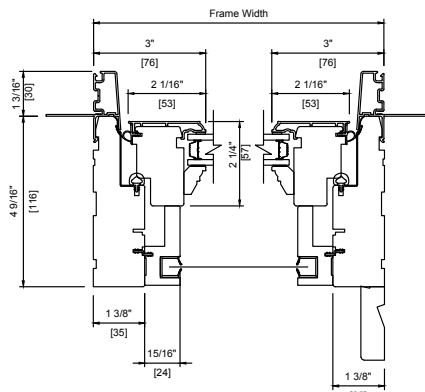
METAL CLAD DOUBLE RETRACTABLE SCREEN
