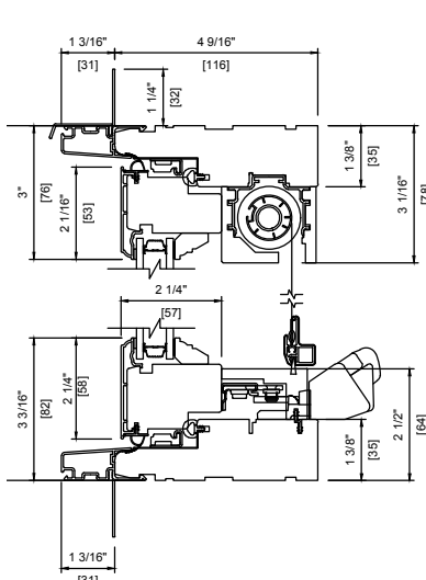
METAL CLAD DOUBLE 4 9/16" (116 mm) RETRACTABLE SCREEN
