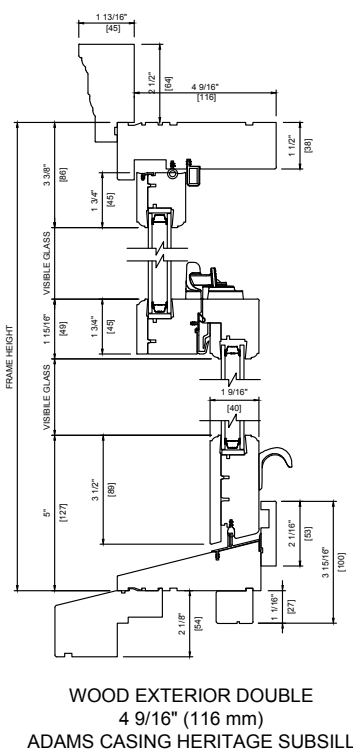
Head & Sill Detail
