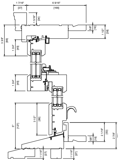
WOOD EXTERIOR TRIPLE 6 9/16" (166 mm) 2" BRICKMOULD STANDARD SUBSILL
