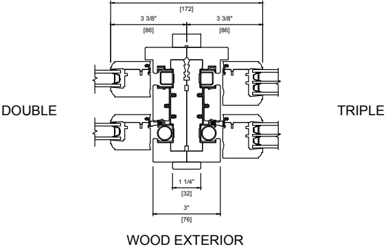
Mull Detail
