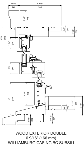
Head & Sill Detail
