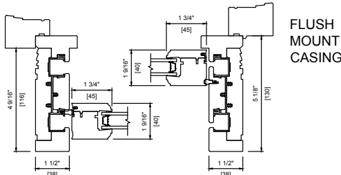
WOOD EXTERIOR DOUBLE 4 9/16" (116 mm) + 5 1/8" (130 mm) 2" BRICKMOULD
