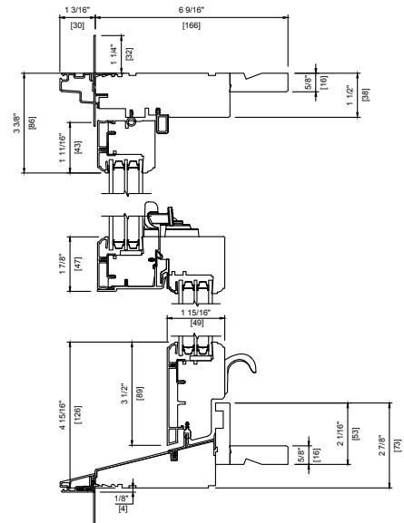
METAL CLAD TRIPLE 6 9/16" (166 mm) MULTILITE SILL NOSE
