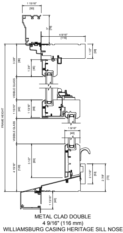
Head & Sill Detail
