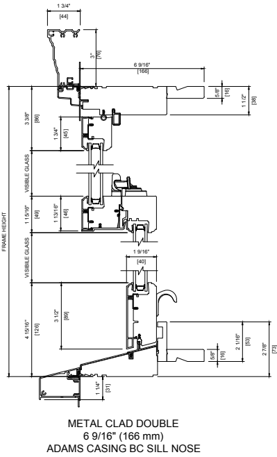
Head & Sill Detail
