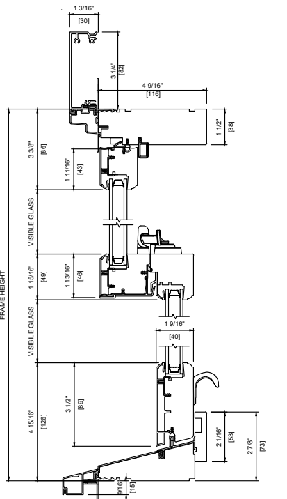
METAL CLAD DOUBLE 4 9/16" (116 mm) 3 1/2" FLAT CASING STANDARD SILL NOSE
