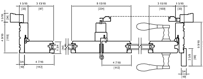
WOOD EXTERIOR DOUBLE TWO PANEL 2" BRICKMOULD SQUARE STOP
