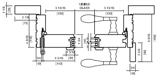
WOOD EXTERIOR TRIPLE ONE PANEL 3 1/2" FLAT CASING TRIPLE GLAZING STOP
