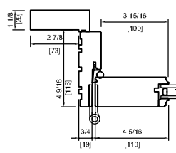
WOOD EXTERIOR DOUBLE CAMBERTOP 3 1/2" FLAT CASING
