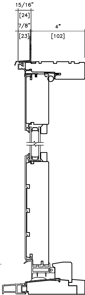
OUTSWING TERRACE/FRENCH TERRACE - STANDARD STILE
