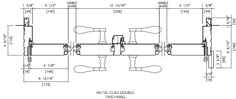
METAL CLAD DOUBLE TWO PANEL
