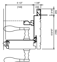
METAL CLAD DOUBLE 6 9/16" (166 mm ) FULL JAMB
