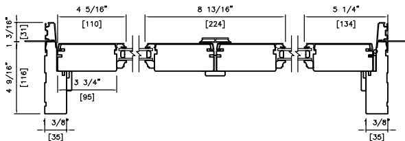
METAL CLAD STANDARD STILE 4 5/16" (110mm) STILES 2-PANEL
