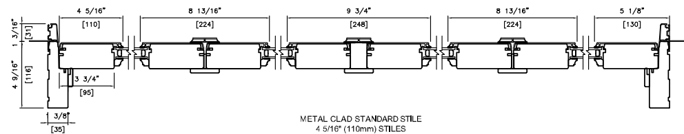
METAL CLAD NARROW STILE 3" (75mm) STILES
