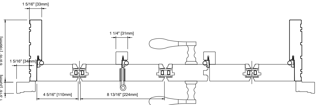
WOOD EXTERIOR - THREE WIDE 6 9/16" (166 mm) JAMB
