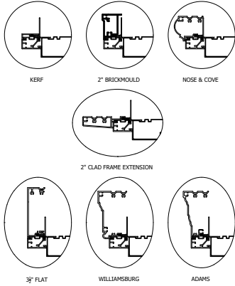
Casing
