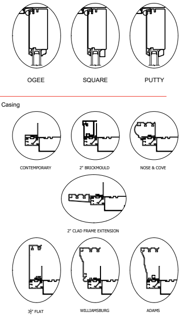
GLAZING STOP PROFILES
