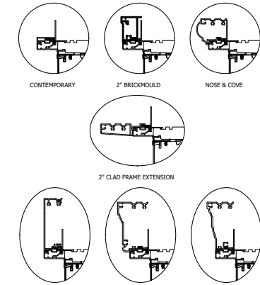
Casing
