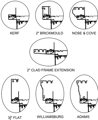
CASING
