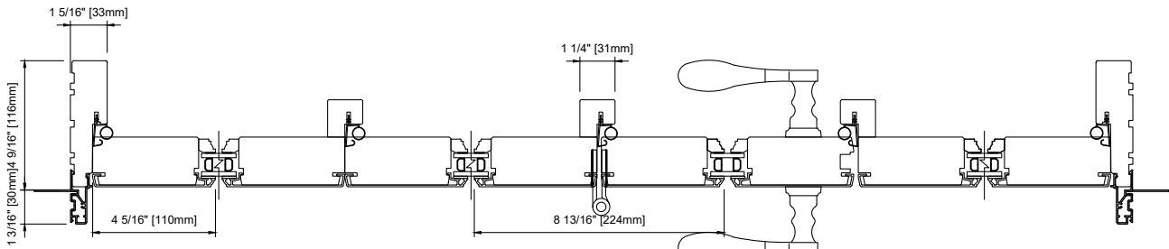
METAL CLAD - THREE WIDE 4 9/16" (116 mm) JAMB
