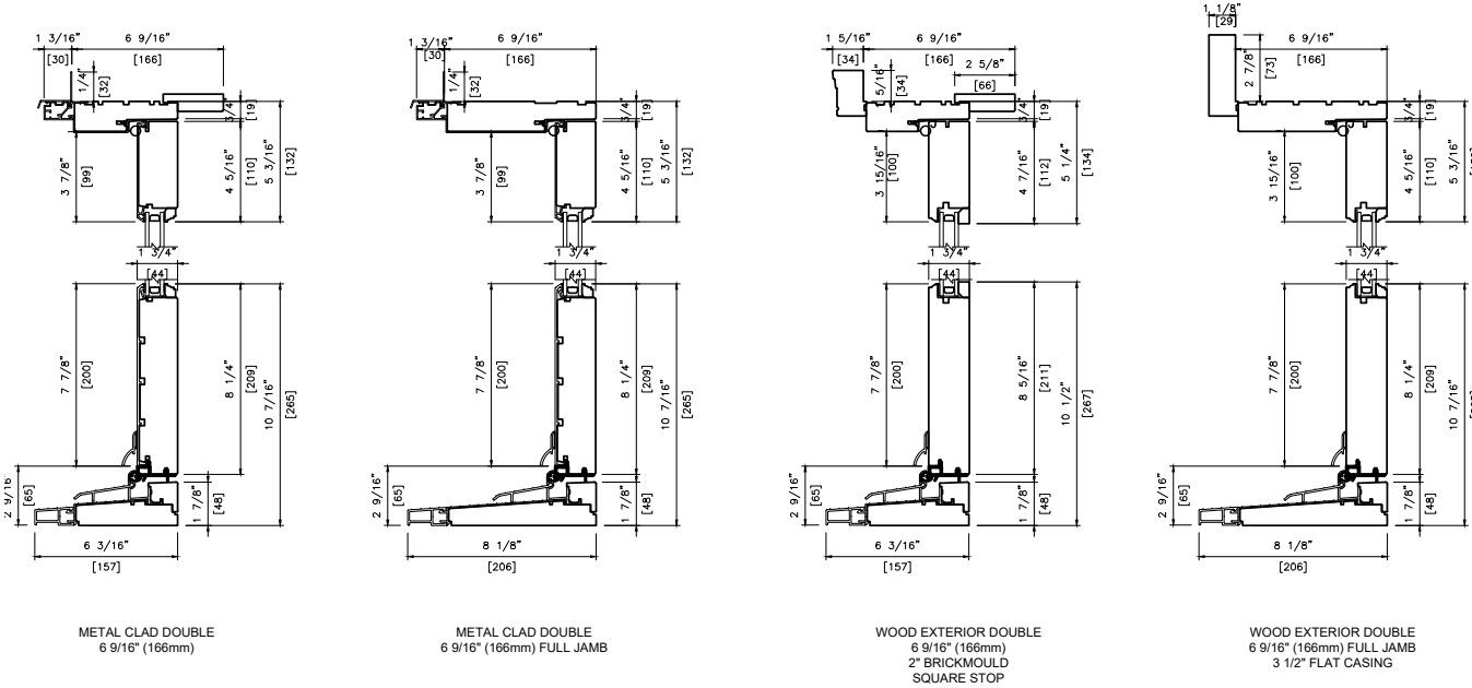
HEAD & SILL DETAIL
