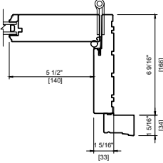
WOOD EXTERIOR DOUBLE 6 9/16" FULL JAMB 2" BRICKMOULD
