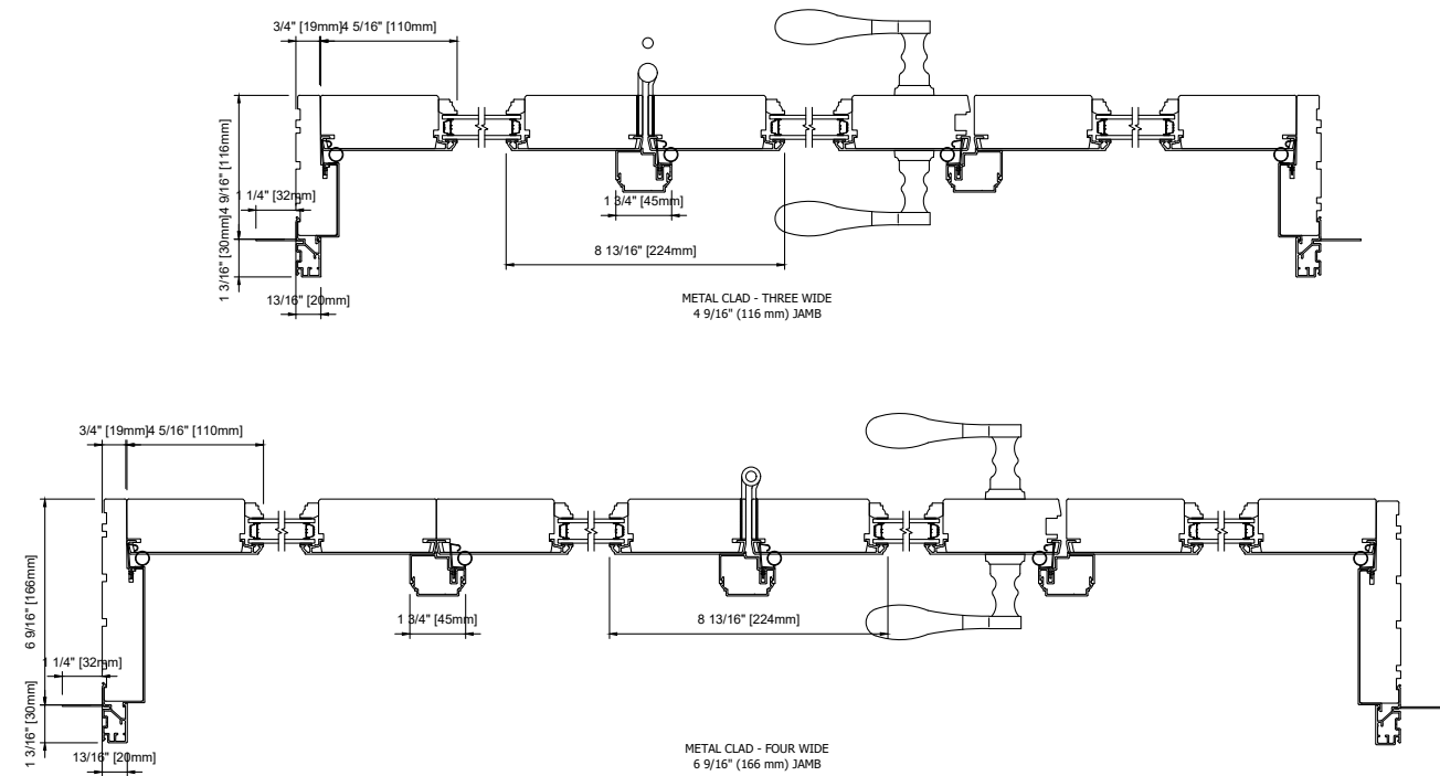
PLAN VIEW
