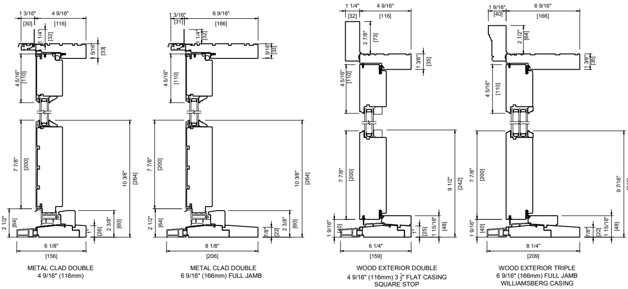
HEAD & SILL DETAILS
