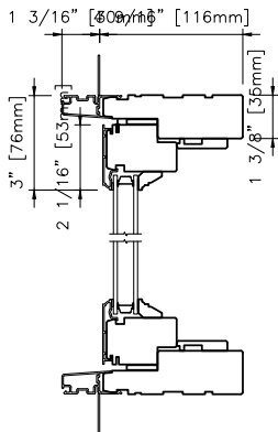
METAL CLAD DOUBLE 2 1/16" (53mm) RAILS
