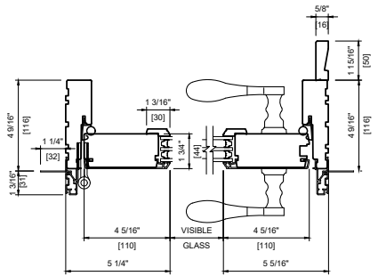
METAL CLAD TRIPLE ONE PANEL TRIPLE GLAZING STOP
