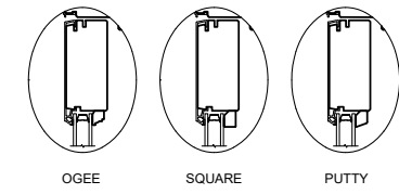
Casing
