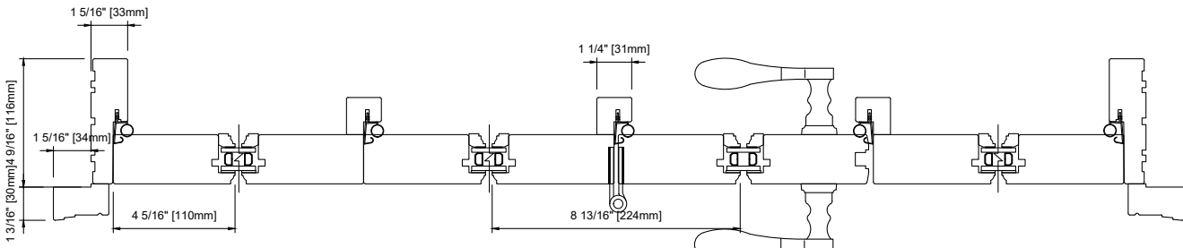
WOOD EXTERIOR - FOUR WIDE 4 9/16" (116 mm) JAMB
