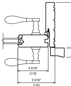
WOOD EXTERIOR DOUBLE 6 9/16" (166 mm) FULL JAMB 2" BRICKMOULD
