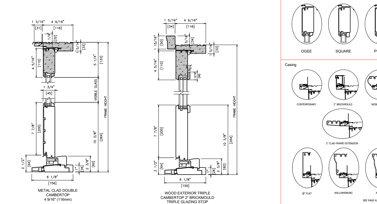
GLAZING STOP PROFILES
