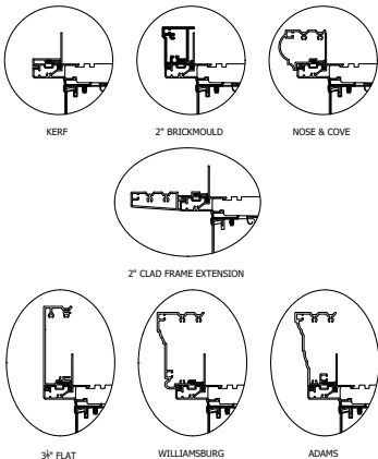
Casing
