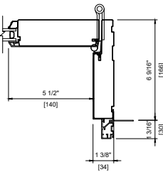
METAL CLAD DOUBLE 6 9/16" FULL JAMB
