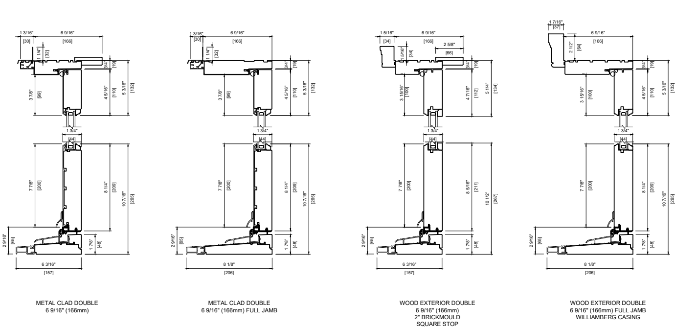
HEAD & SILL DETAIL
