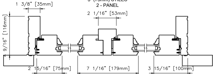
METAL CLAD DOUBLE 3" (75mm) STILES 2 - PANEL
