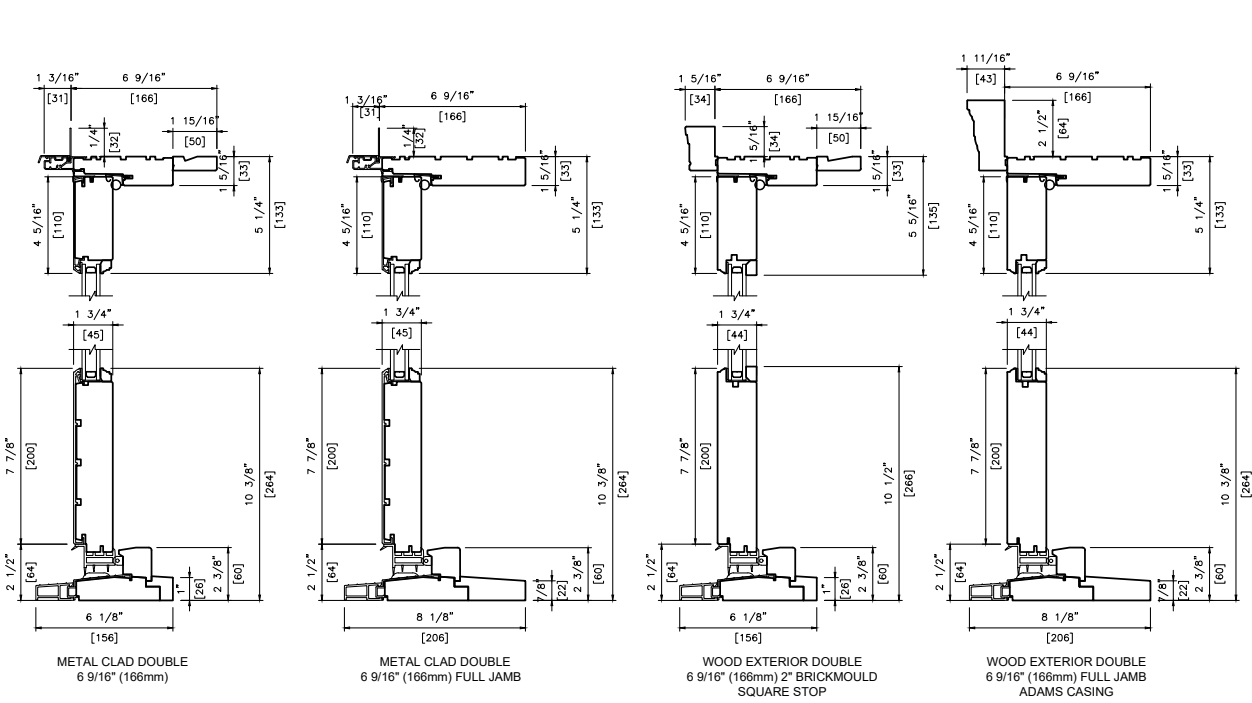
HEAD & SILL DETAILS
