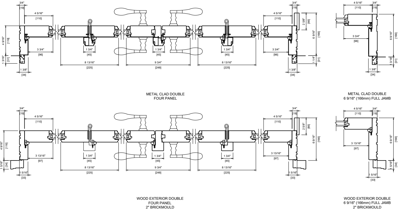
PLAN VIEW
