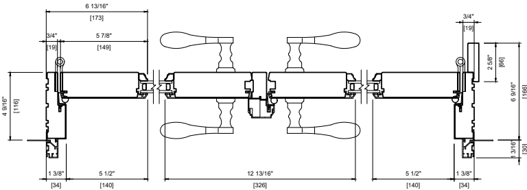
PLAN VIEW INSWING
