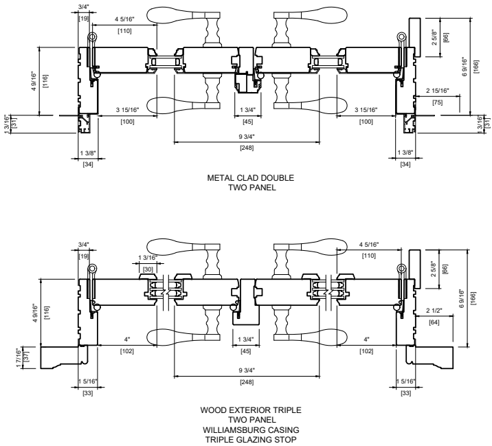
GLAZING STOP PROFILES
