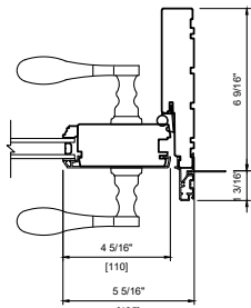
METAL CLAD DOUBLE 6 9/16" (166 mm) FULL JAMB
