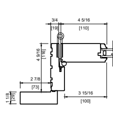
WOOD EXTERIOR DOUBLE TRIPLE CAMBERTOP 3 1/2" FLAT CASING
