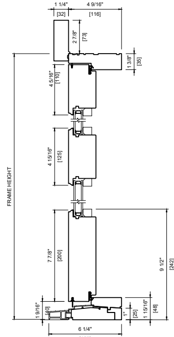
WOOD EXTERIOR with MIDRAIL 4 9/16" (116mm)
