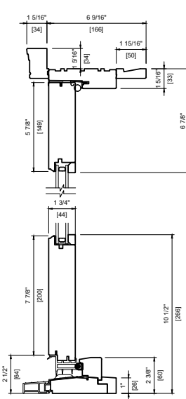
WOOD EXTERIOR DOUBLE 6 9/16" (166mm) 2" BRICKMOULD SQUARE STOP
