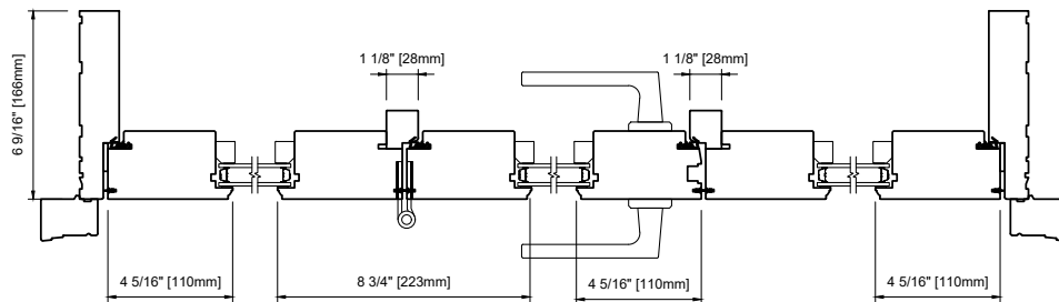
WOOD EXTERIOR DOUBLE 3 WIDE 2 BRICKMOULD, SQUARE STOP
