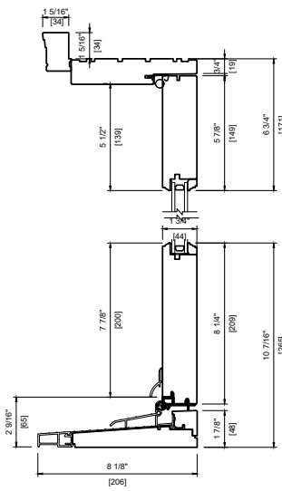
WOOD EXTERIOR DOUBLE 6 9/16" (166mm) FULL JAMB 2" BRICKMOULD
