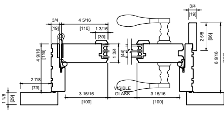
WOOD EXTERIOR TRIPLE ONE PANEL 3 1/2" FLAT CASING TRIPLE GLAZING STOP
