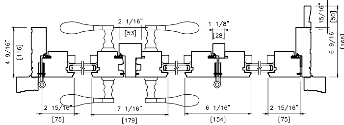
WOOD EXTERIOR DOUBLE THREE PANEL 2 IN. BRICKMOULD SQUARE STOP
