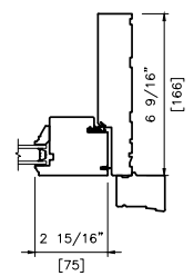
METAL CLAD DOUBLE 6 9/16" (166 mm) FULL JAMB
