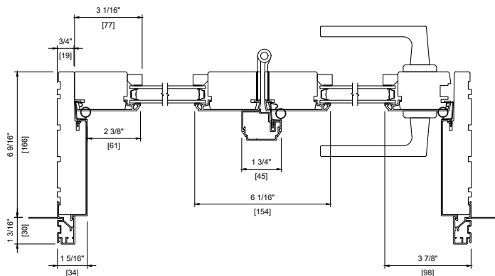
METAL CLAD DOUBLE TWO PANEL 6 \frac{5}{8} " (166 mm)
