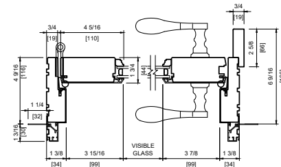
METAL CLAD DOUBLE ONE PANEL
