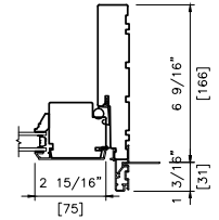
METAL CLAD DOUBLE 6 9/16" (166 mm) FULL JAMB
