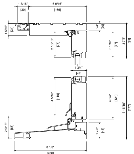
METAL CLAD DOUBLE 6 \frac{5}{8} " (166 mm) FULL JAMB
