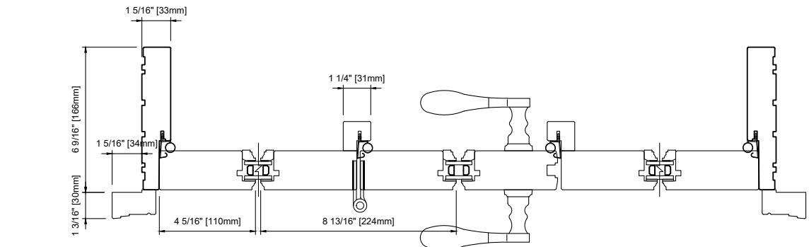
WOOD EXTERIOR - THREE WIDE 6 9/16" (166 mm) JAMB
