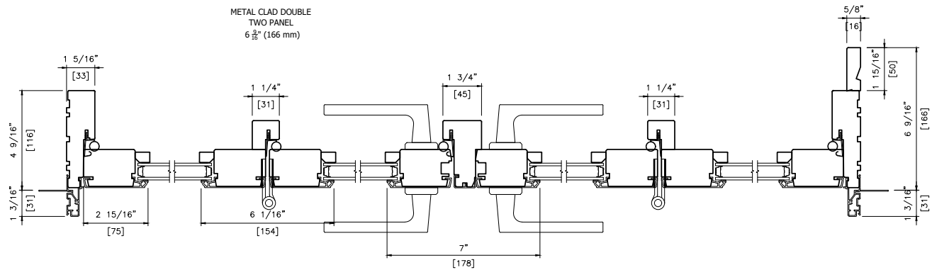
METAL CLAD DOUBLE FOUR PANEL 4 5/8" / 6 3/8" (116 mm / 166 mm)
