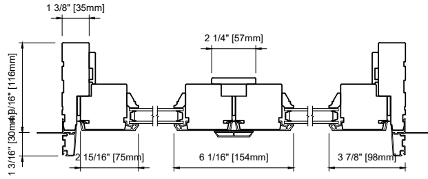
METAL CLAD DOUBLE 2 15/16" (75mm) STILES 2 - PANEL
