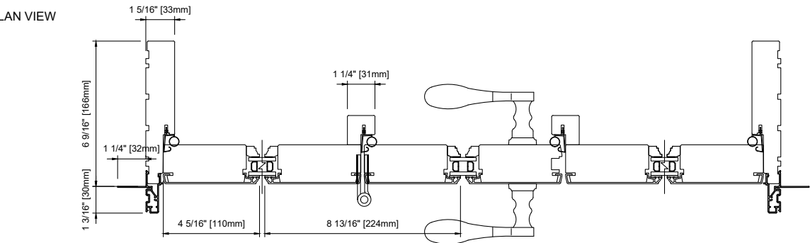
METAL CLAD - THREE WIDE 4 9/16" (116 mm) JAMB
