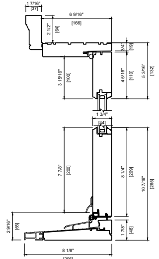
WOOD EXTERIOR DOUBLE 6 9/16" (166mm) FULL JAMB WILLIAMSBERG CASING
