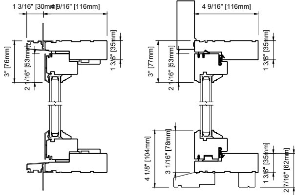
METAL CLAD DOUBLE 2 1/16" (53mm) RAILS
