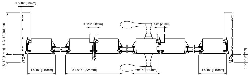
METAL CLAD DOUBLE 3 WIDE
