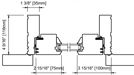
METAL CLAD DOUBLE 2 15/16" (75mm) STILES
