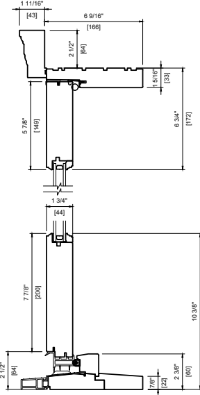
WOOD EXTERIOR DOUBLE 6 9/16" (166mm) FULL JAMB ADAMS CASING
