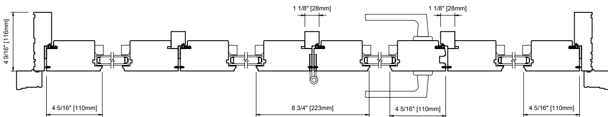
WOOD EXTERIOR DOUBLE 4 WIDE 2 BRICKMOULD, SQUARE STOP
