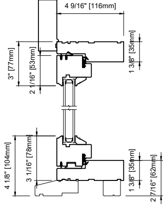
WOOD EXTERIOR DOUBLE 2 1/16" (53mm) RAILS
