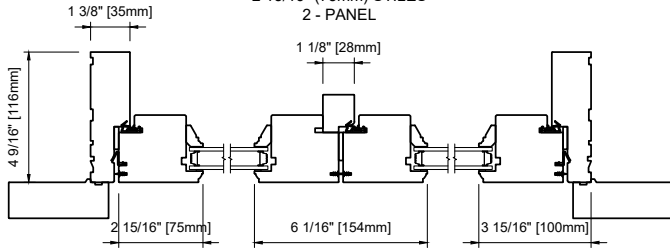
WOOD EXTERIOR DOUBLE 2 15/16" (75mm) STILES 2 - PANEL
