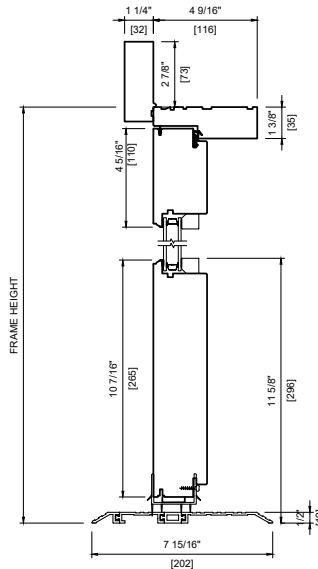
WOOD EXTERIOR with Flat Sill and Tall Bottom Rail 4 9/16" (116mm)
