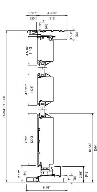
METAL CLAD with MIDRAIL 4 9/16" (116mm)
