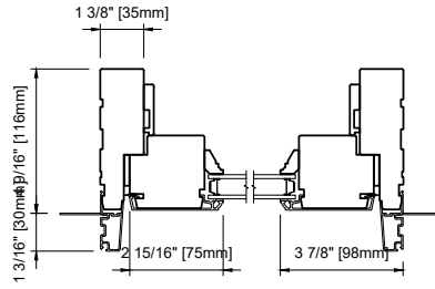
METAL CLAD DOUBLE 2 15/16" (75mm) STILES
