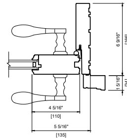
WOOD EXTERIOR DOUBLE 6 9/16" (166 mm) FULL JAMB 2" BRICKMOULD
