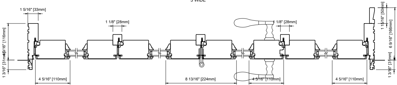
METAL CLAD DOUBLE 4 WIDE
