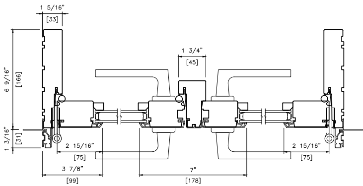
METAL CLAD DOUBLE TWO PANEL 6 3/8" (166 mm)
