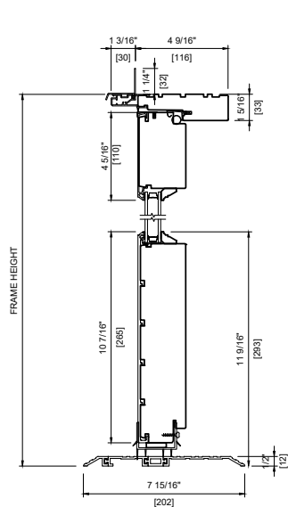
METAL CLAD with Flat Sill and Tall Bottom Rail 4 9/16" (116mm)
