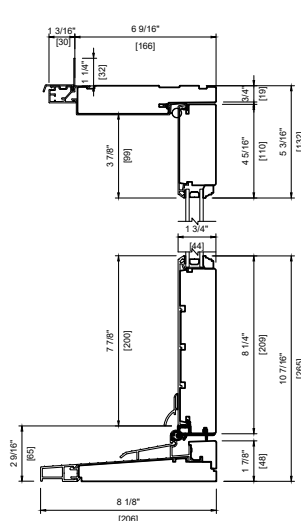
METAL CLAD DOUBLE 6 9/16" (166mm) FULL JAMB
