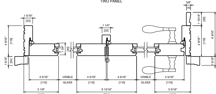
WOOD EXTERIOR DOUBLE TWO PANEL 2 BRICKMOULD SQUARE STOP
