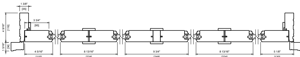
WOOD EXTERIOR STANDARD STILE 4 5/16" (110mm) STILES
