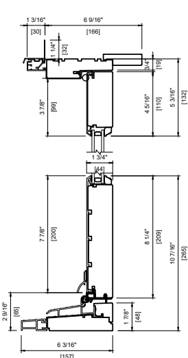
METAL CLAD DOUBLE 6 9/16" (166mm)
