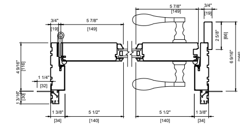
METAL CLAD DOUBLE ONE PANEL
