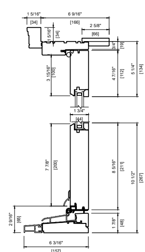
WOOD EXTERIOR DOUBLE 6 9/16" (166mm) 2" BRICKMOULD SQUARE STOP
