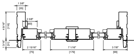
METAL CLAD NARROW STILE 3" (75mm) STILES
