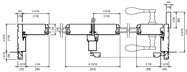
METAL CLAD DOUBLE TWO PANEL
