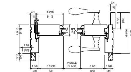
METAL CLAD DOUBLE ONE PANEL
