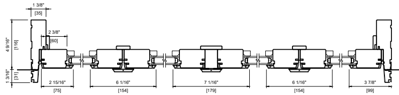
METAL CLAD NARROW STILE 3" (75mm) STILES
