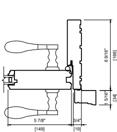
METAL CLAD DOUBLE 6 9/16" FULL JAMB
