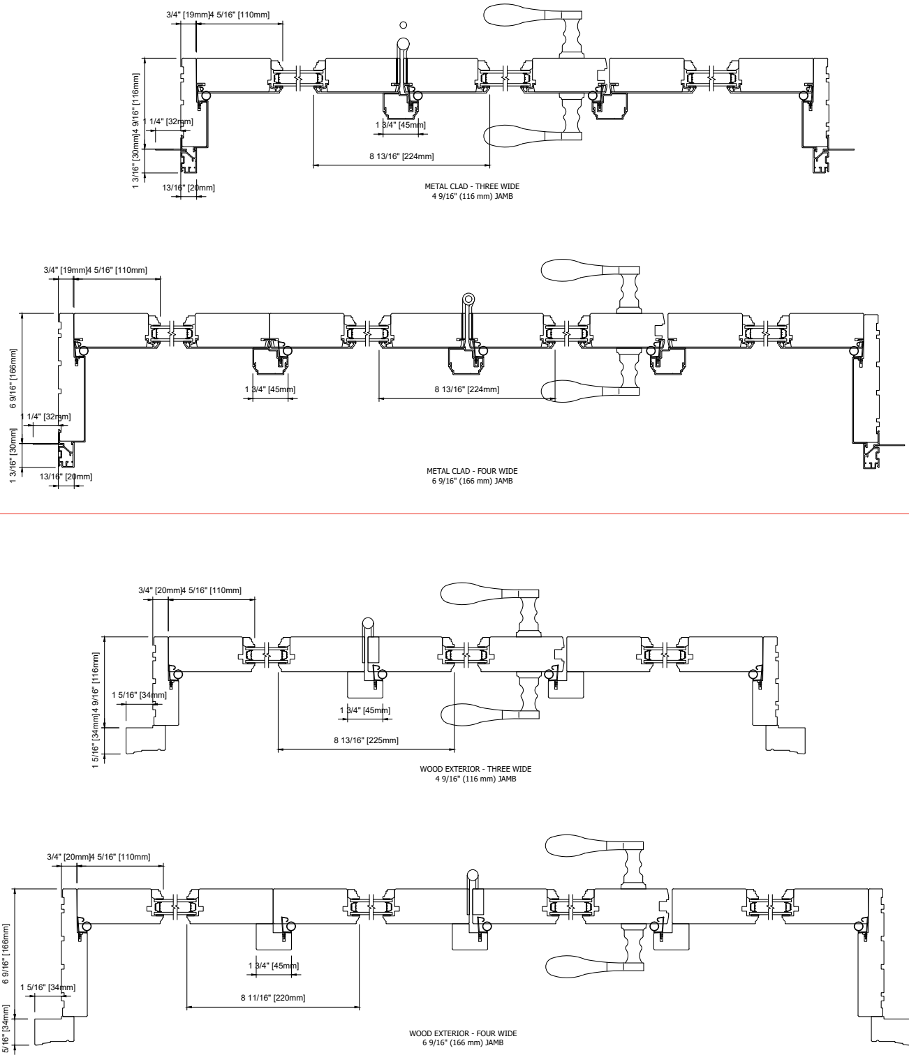
PLAN VIEW
