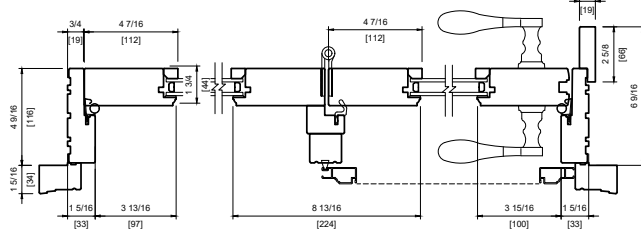
WOOD EXTERIOR DOUBLE TWO PANEL 2" BRICKMOULD SQUARE STOP
