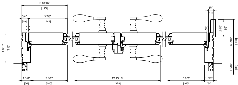
PLAN VIEW INSWING
