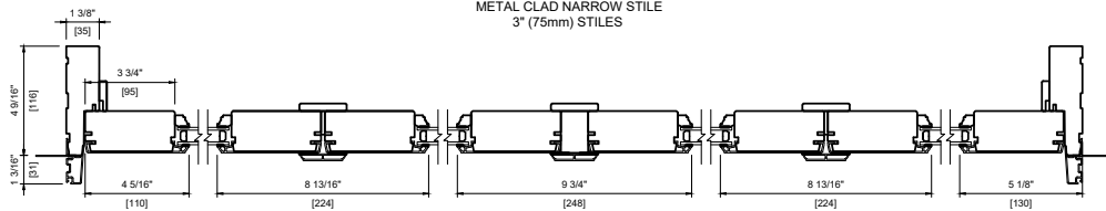
METAL CLAD STANDARD STILE 4 5/16" (110mm) STILES
