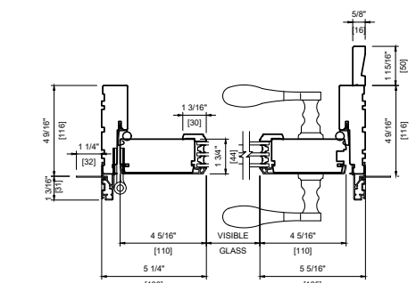
METAL CLAD TRIPLE ONE PANEL TRIPLE GLAZING STOP
