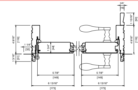
METAL CLAD DOUBLE ONE PANEL
