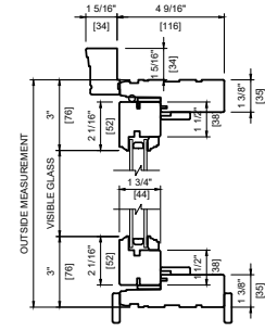
WOOD EXTERIOR DOUBLE 2 1/16" (52mm) RAILS 2" BRICKMOLD
