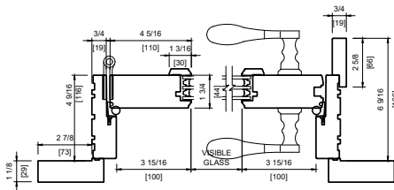
METAL CLAD DOUBLE ONE PANEL
