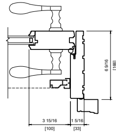
METAL CLAD DOUBLE 6 9/16" (166 mm) FULL JAMB
