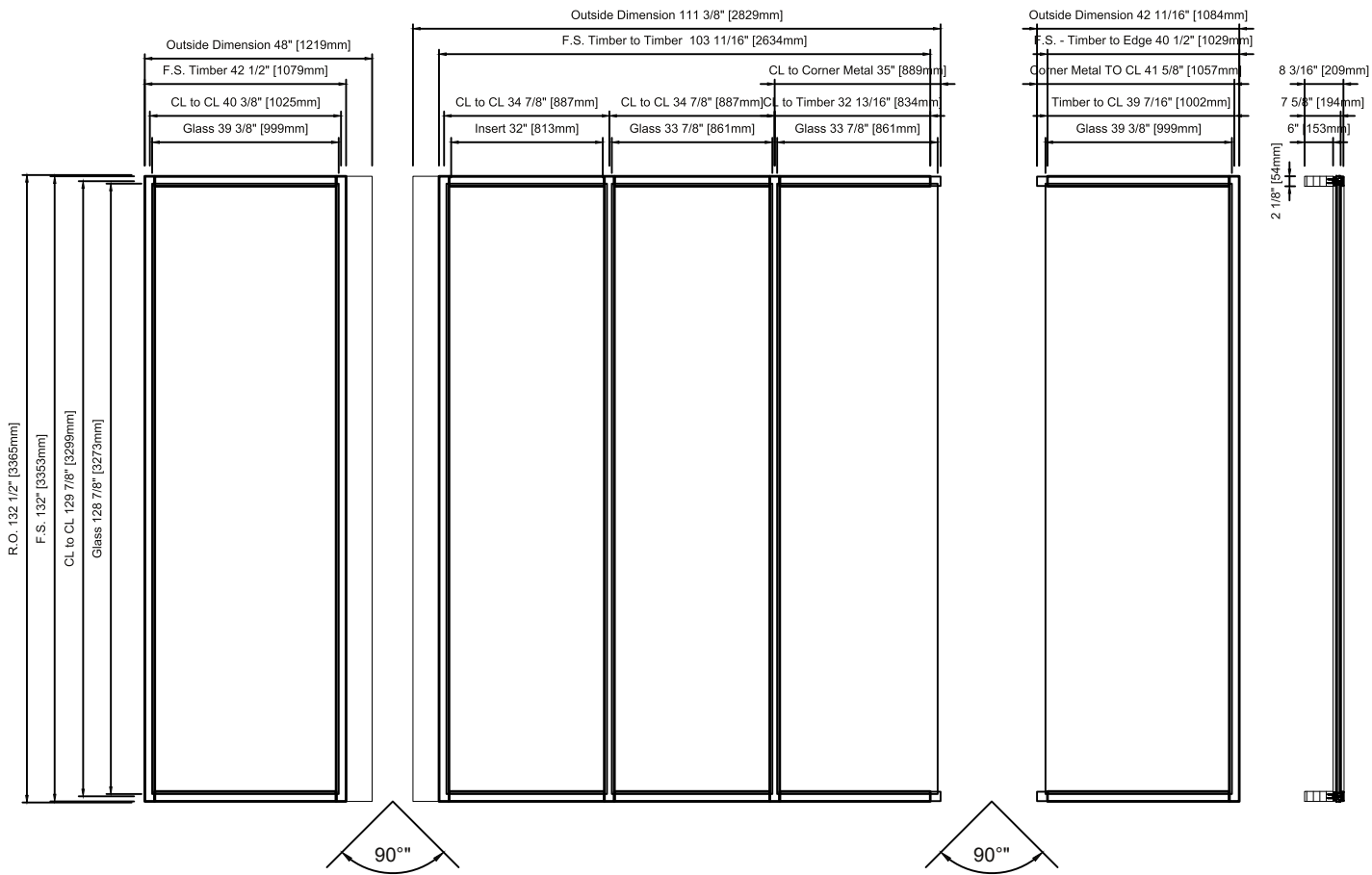
Plan View
