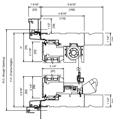
METAL CLAD DOUBLE 6 9/16" (166 mm) 2" BRICKMOULD WITH STANDARD SILL NOSE RETRACTABLE SCREEN
