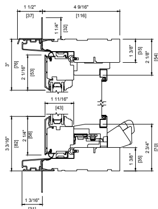
METAL CLAD DOUBLE 4 9/16" (116 mm) STANDARD SCREEN
