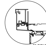
2" BRICKMOLD
