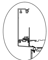
3 1/2" FLAT
