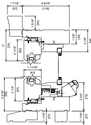
WOOD EXTERIOR DOUBLE 4 9/16" (116 mm) 2" BRICKMOULD WITH STANDARD SUBSILL STANDARD SCREEN
