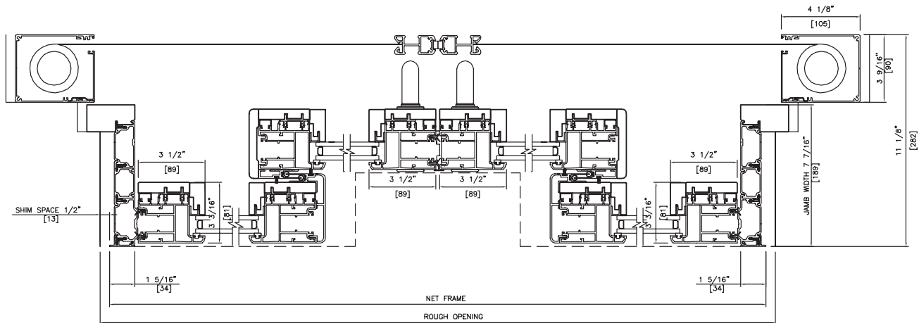
OX-XO STEPPED HEAD WITH SCREEN
