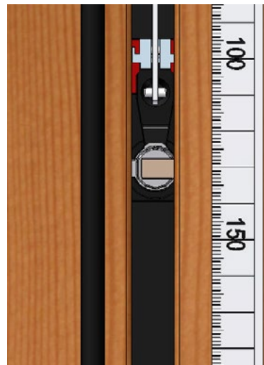
Opposite Jamb
