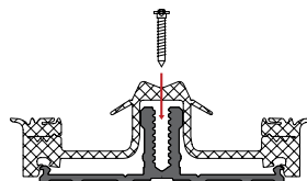
Step 3-7 Screw into the "V-Dent" through the center of the rubber gasket.
